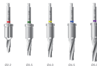
Step Drill
